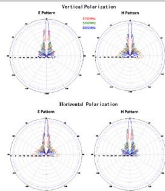
Antenna Pattern
